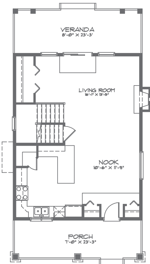
MAIN FLOOR PLAN AREA: 698 SQFT.
