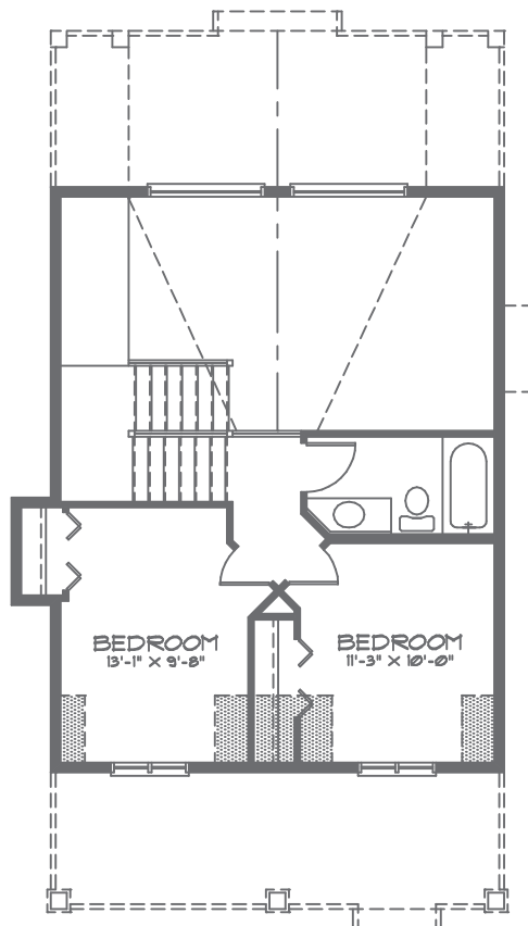
UPPER FLOOR PLAN AREA: 341 SQFT.
