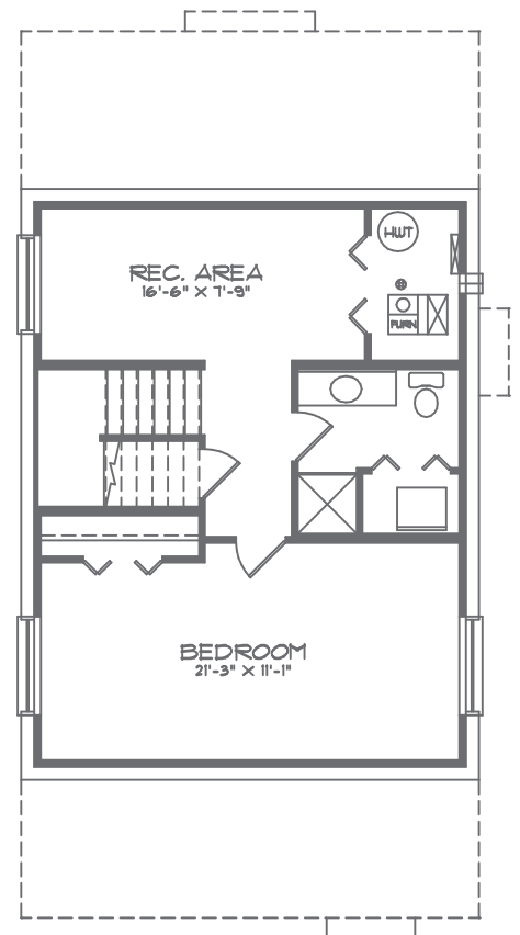
BSMT. FLOOR PLAN AREA: 560 SQFT.
