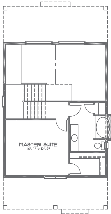
UPPER FLOOR PLAN AREA: 339 SQ.FT.
