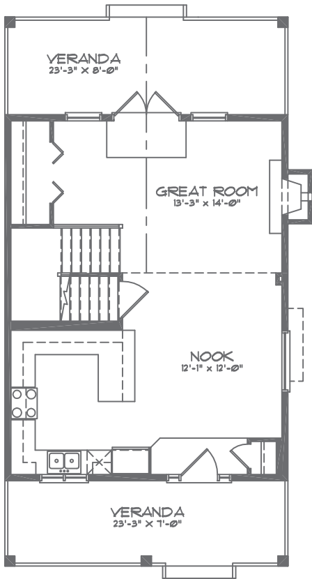
MAIN FLOOR PLAN AREA: 698 SQ.FT.
