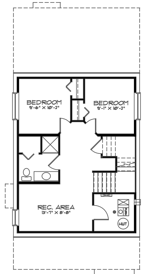
BSMT. FLOOR PLAN AREA: 484 SQFT.
