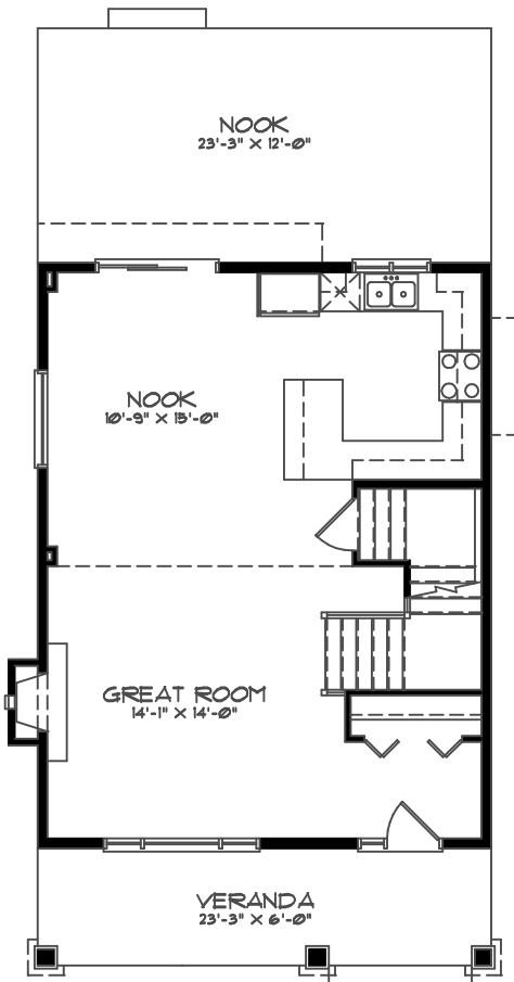
MAIN FLOOR PLAN AREA: 698 SQFT.
